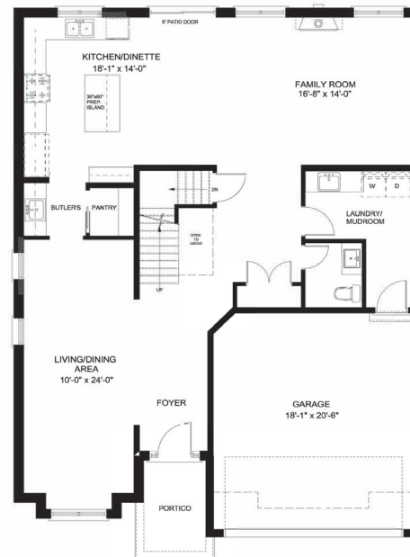
GROUND FLOOR PLAN 1,374sf
